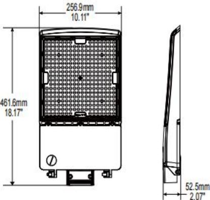
200W
