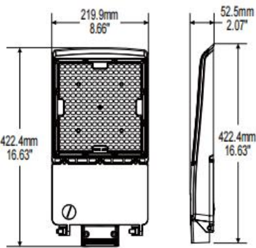
100W&150W
